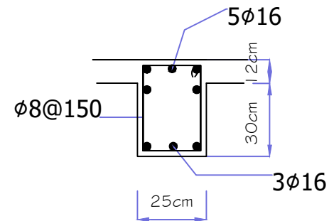
SEC.X-X
