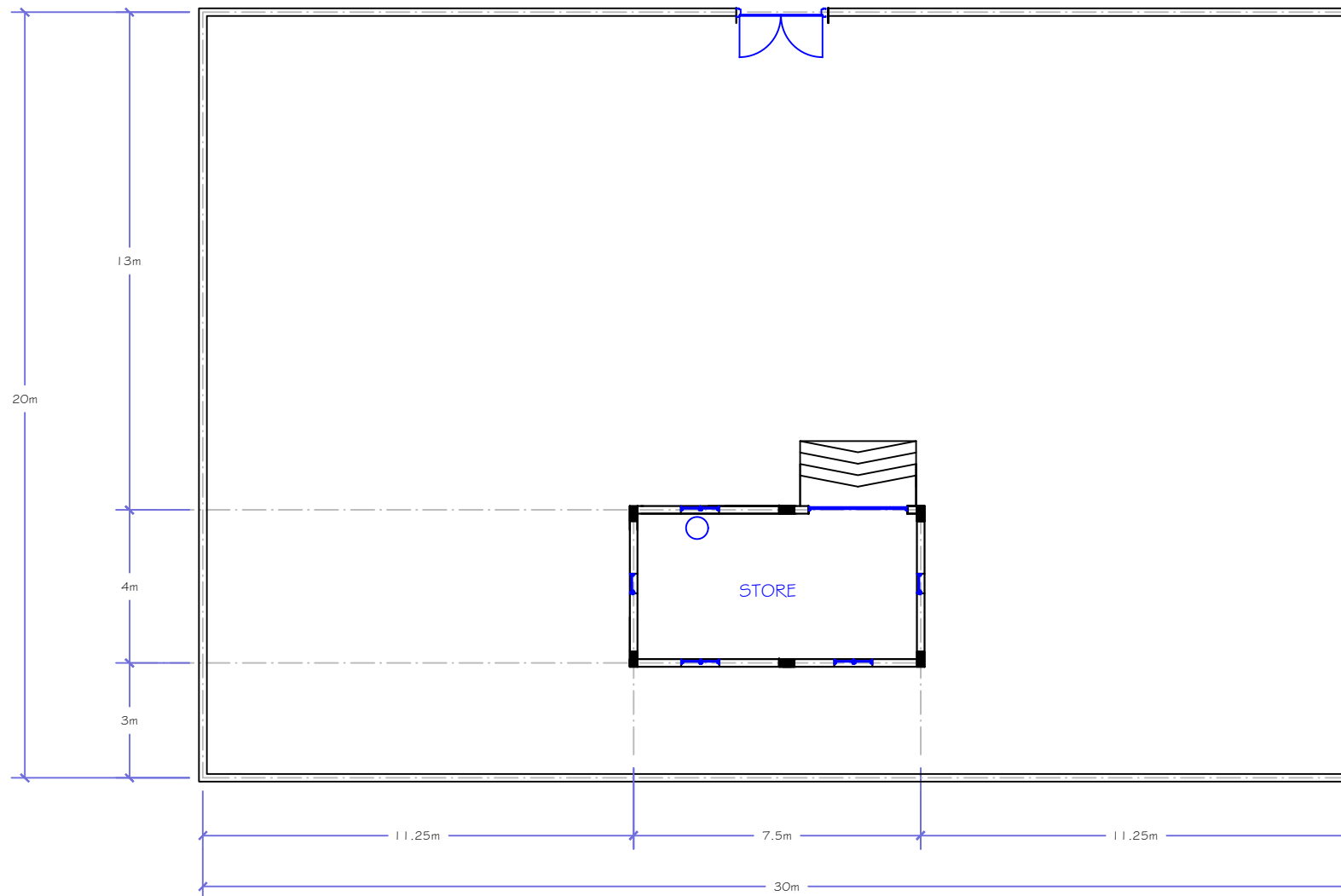
LAYOUT PLAN
