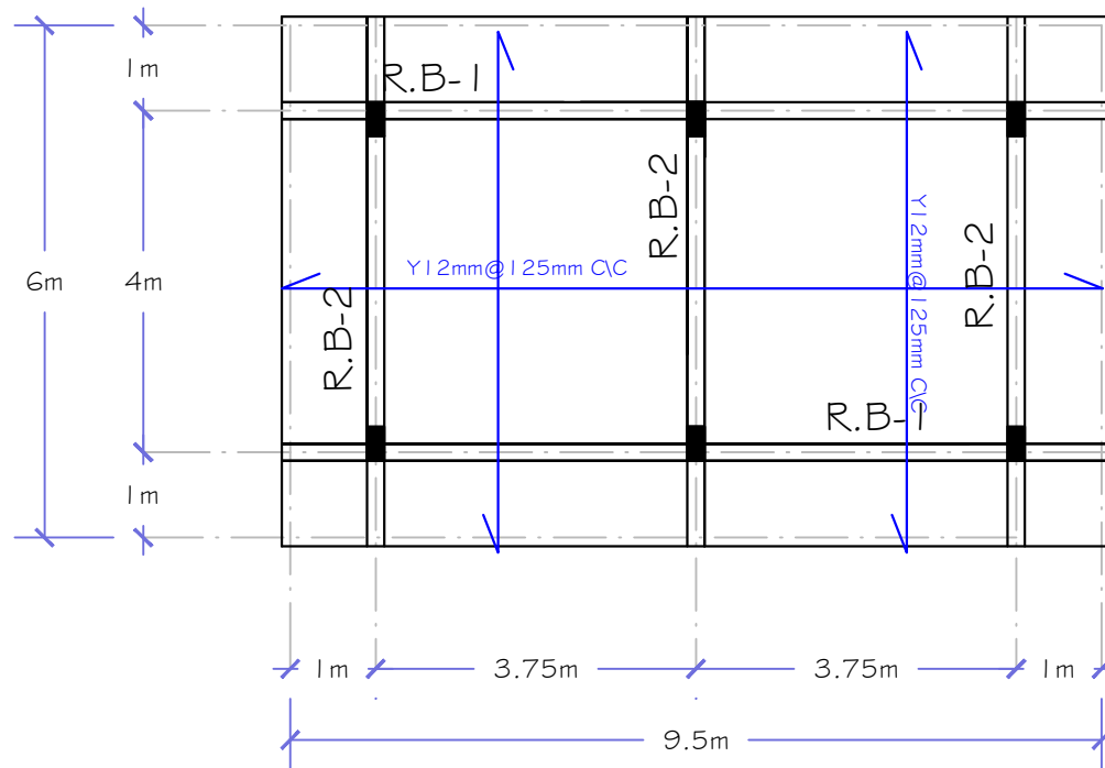
GROUND FLOOR ROOF BEAM & SLAP PLAN
