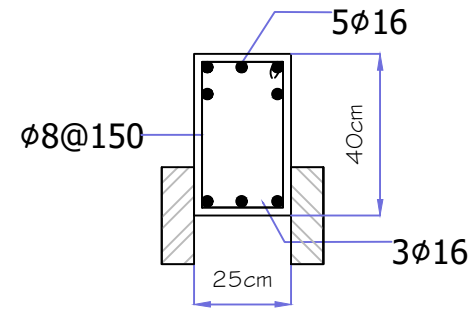
SEC.5-5
