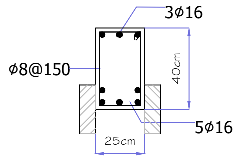
SEC.4-4
