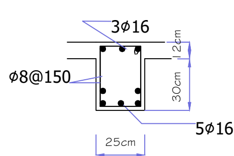
SEC.Y-Y
