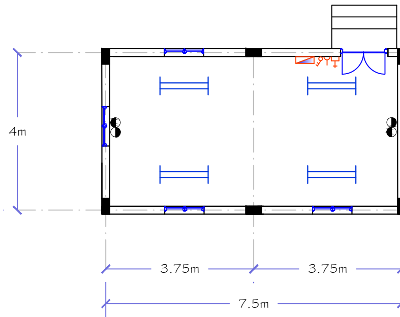
ELECTRICITY PLAN
